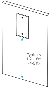
Figure 2 AcuTEMS WP Typical Mounting Location
