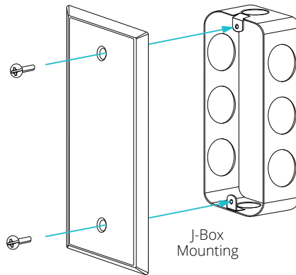
Figure 5 AcuTEMS WP Junction Box Mounting
