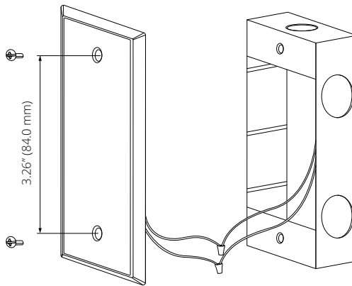
Figure 3 AcuTEMS WP Flying Lead Connection
