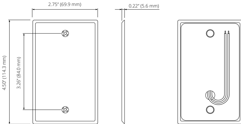
Figure 1 AcuTEMS WP Front and Side Views
