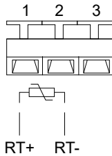
Figure 6 AcuTEMS DM Wiring Terminals for Resistive Output
