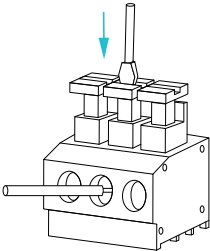
Figure 4 AcuTEMS DM Push Button Terminal Block
