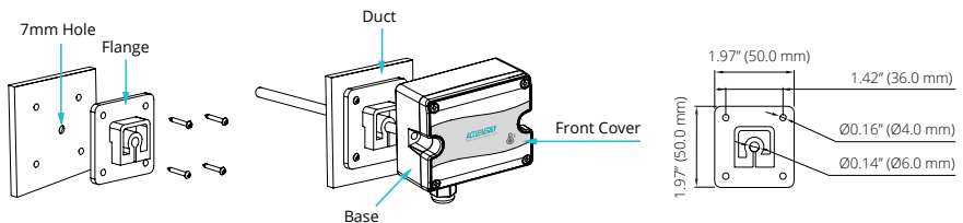
Figure 7 Duct Mount with Flange
