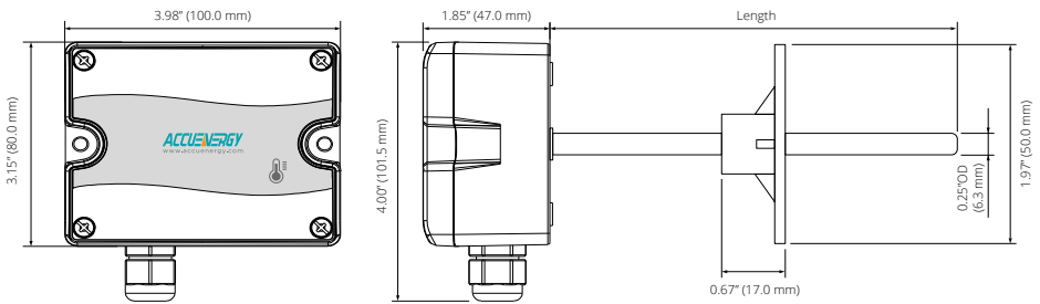
Figure 1 AcuTEMS DM Front and Side Views
