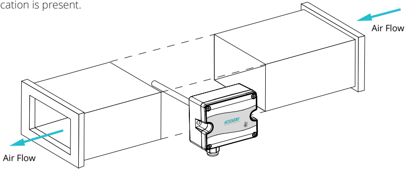
Figure 2 AccuTEMS DM Mounting Location
