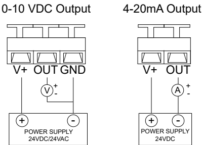
Figure 5 AcuTEMS DM Wiring Terminals for Temperature Transmitter
