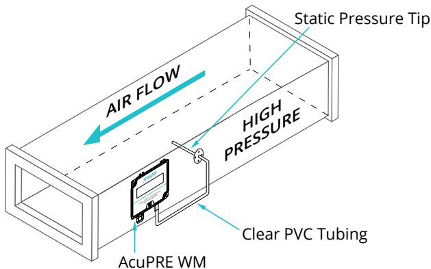
Figure 3 AcuPRE WM Duct Static Pressure Connection
