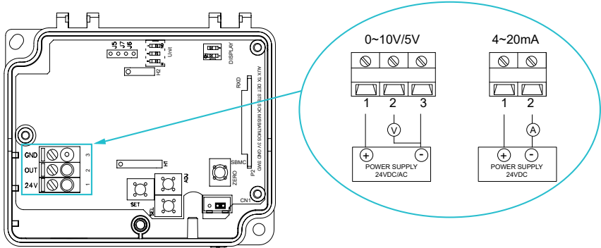
Figure 8 AcuPRE WM Wiring Terminals
