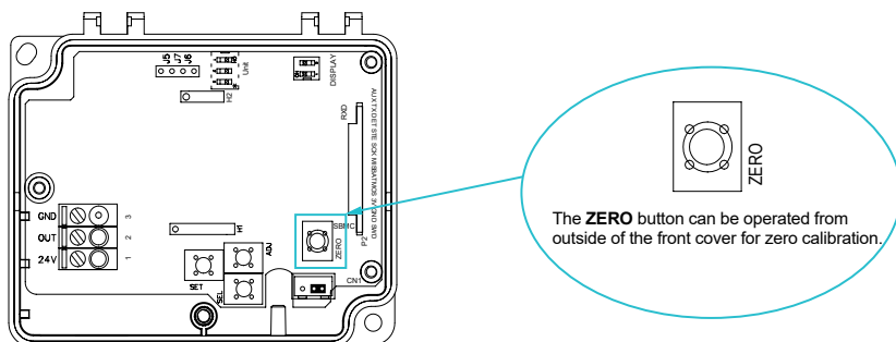
Figure 12 AcuPRE WM Zero Calibration Button
