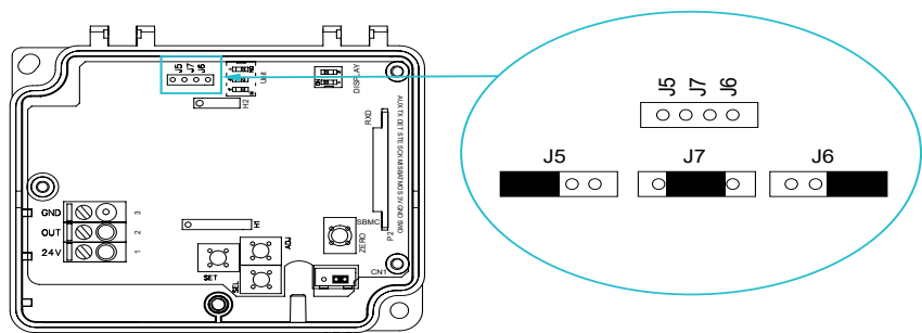
Figure 9 AcuPRE WM Pressure Range Selection Jumpers
