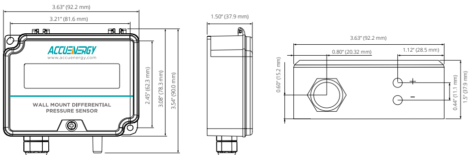
Figure 1 AcuPRE WM Front and Bottom Views
