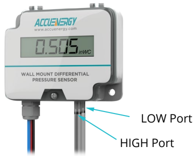
Figure 6 AcuPRE WM HIGH and LOW Pressure Ports
