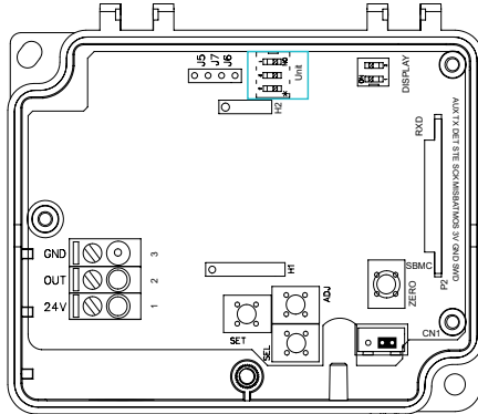
Figure 10 AcuPRE WM Unit Selection DIP Switches
