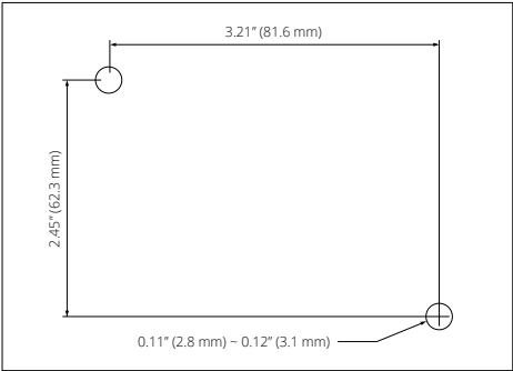
Figure 5 AcuPRE WM Mounting Template
