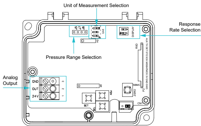
Figure 2 Internal Schematics of AcuPRE WM
