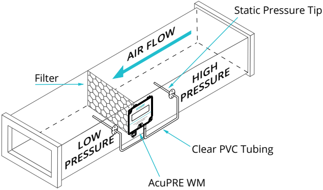
Figure 4 AcuPRE WM Filter Status Detection
