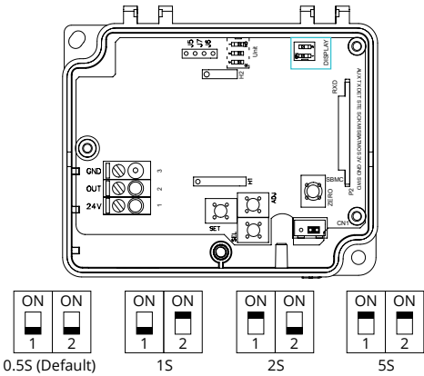
Figure 11 Response Rate Selection DIP Switches
